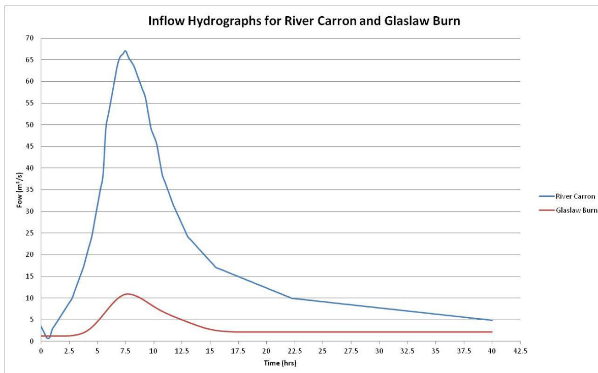
Figure B-2: River Carron and Glaslaw Burn Hydrographs
