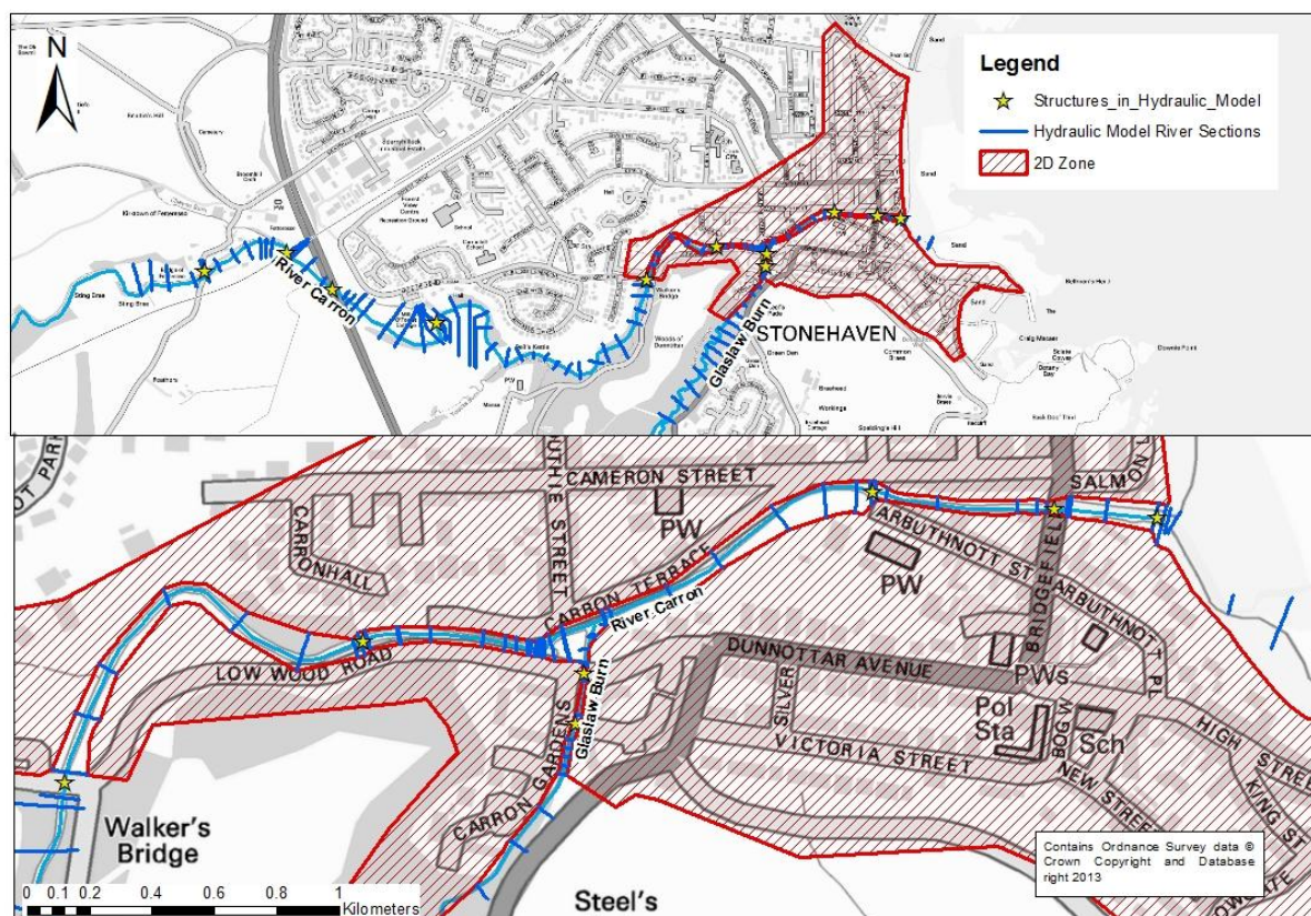
Figure B-1: Hydraulic Model Geometry
