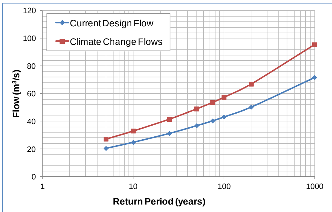
Figure 6-1: Impact of climate change on flood flows
